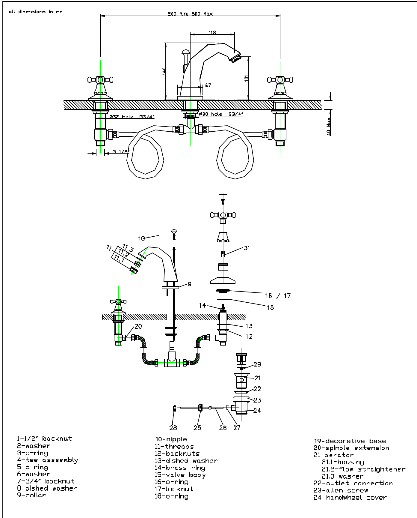
Algarve 3 hole basin mixer
