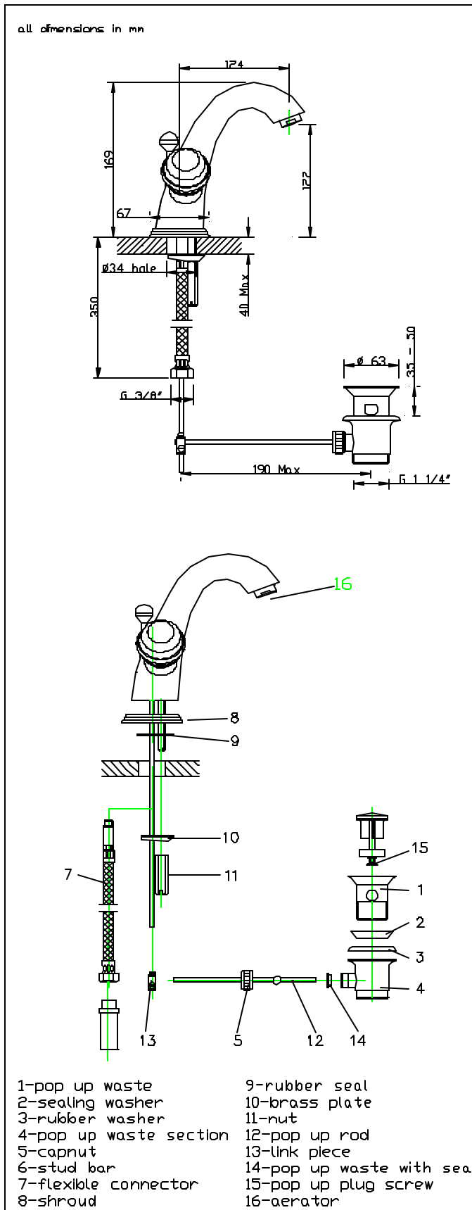
King monobloc basin mixer
